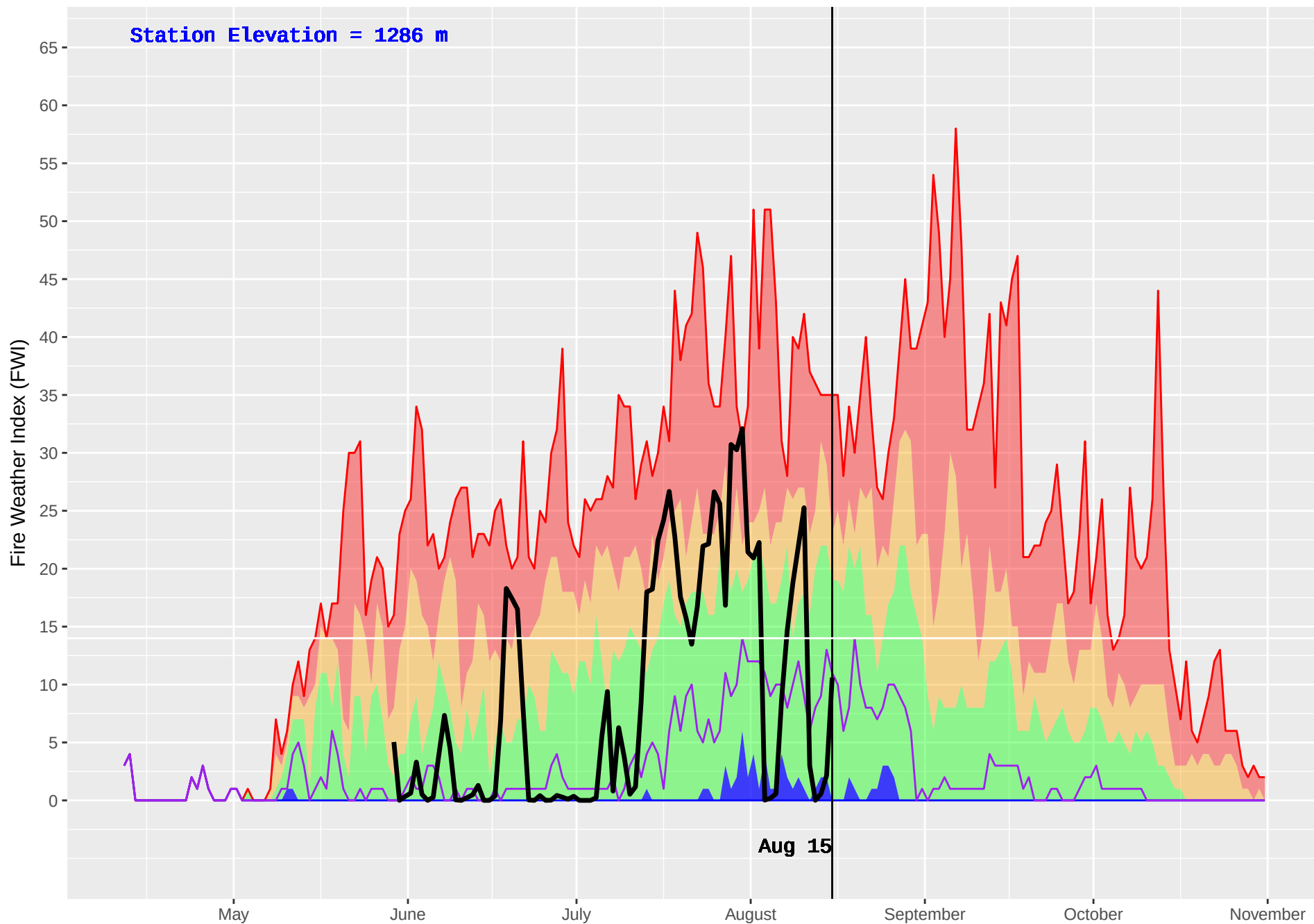
CURWEN CREEK (352) : Historical (1979–2016) and Current (2018) Daily Fire Weather Index (FWI)
