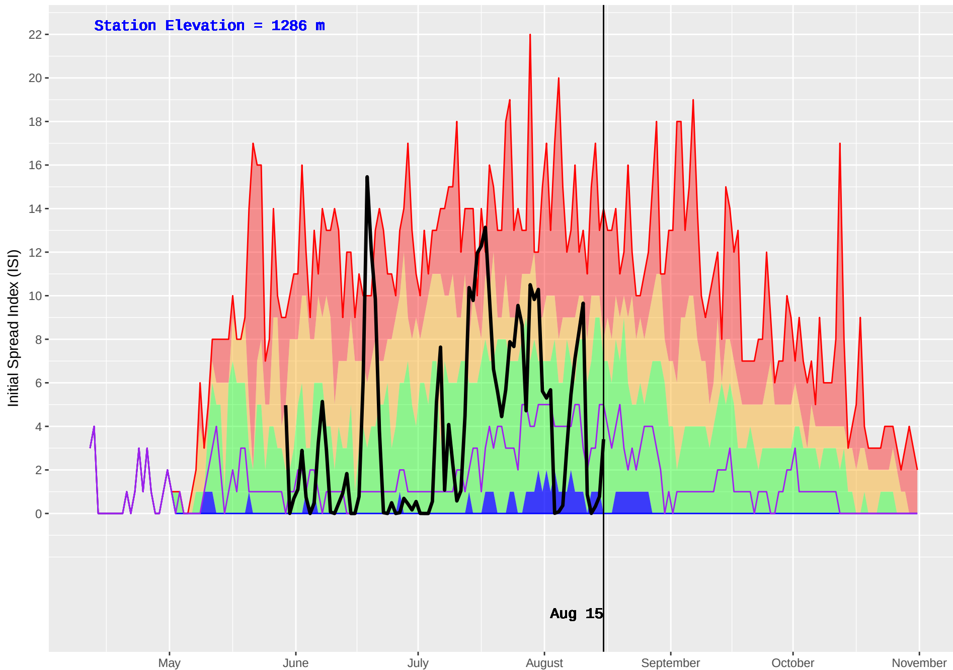
CURWEN CREEK (352) : Historical (1979–2016) and Current (2018) Daily Initial Spread Index (ISI)
